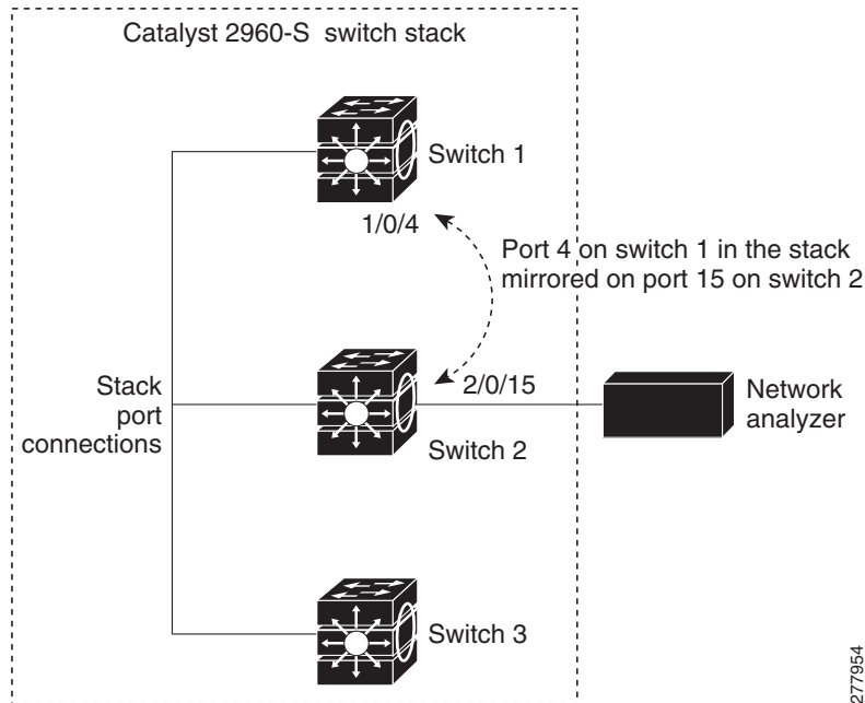
Figure 37-3 Cross-Stack EtherChannel
