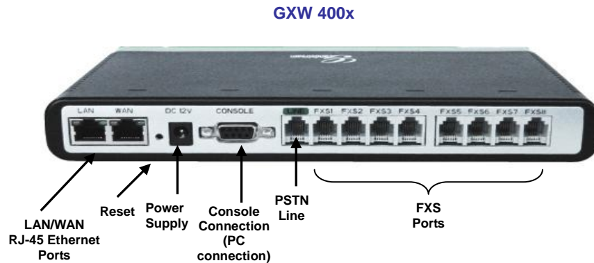
FIGURE 1: DIAGRAM OF GXW4004-8 BACK PANEL
