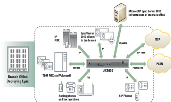
Figure 1: UX1000 offers complete Lync integration to small/mid-sized branches
